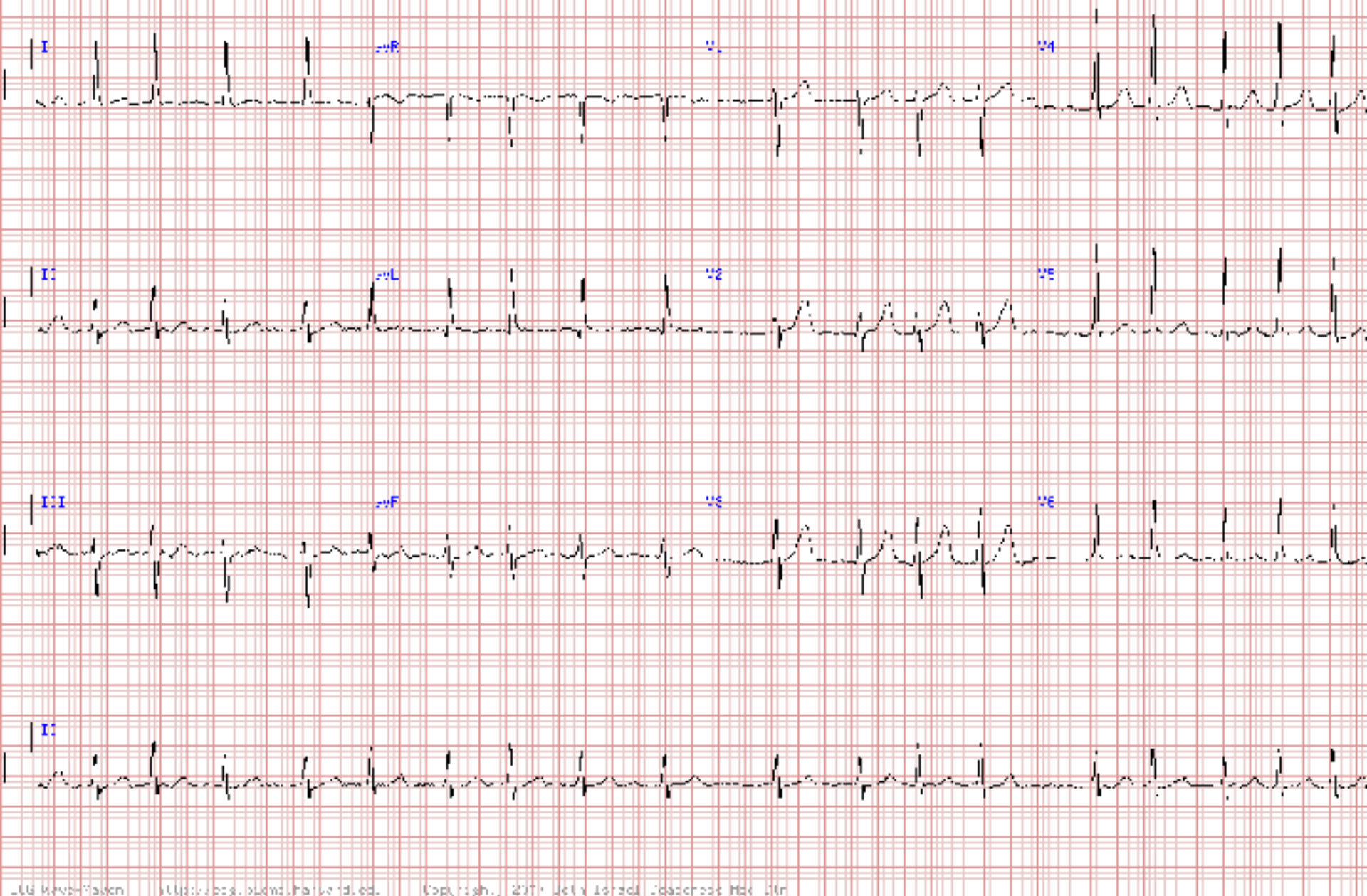
atrial fibrillation
