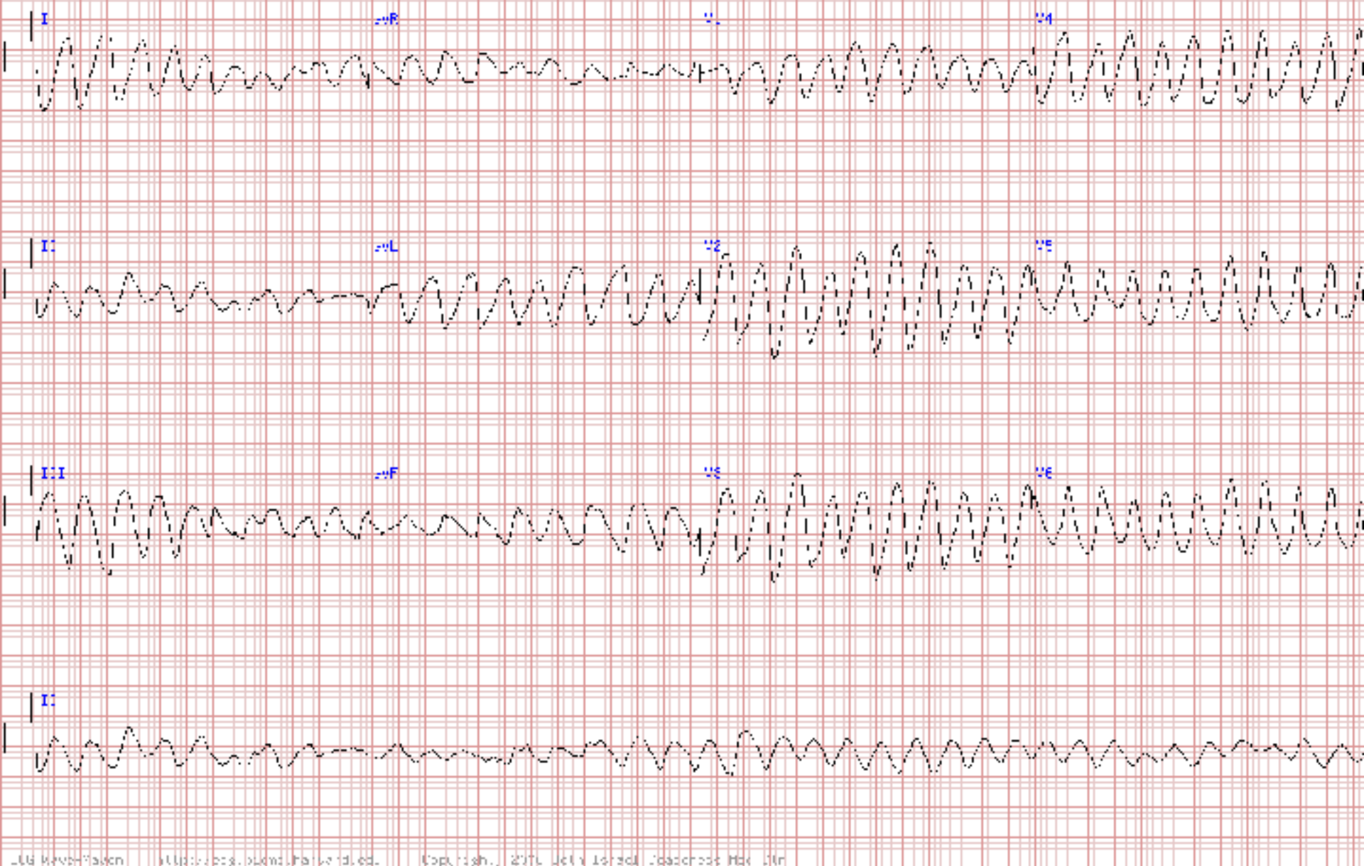
ventricular fibrillation
